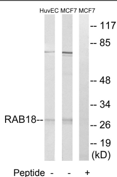
Western blot analysis of extracts from HuvEc cells and MCF-7 cells, using RAB18 antibody.
